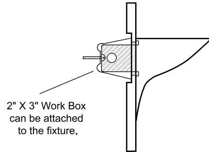
Cross Section of Cut in Box Attached to Fixture
