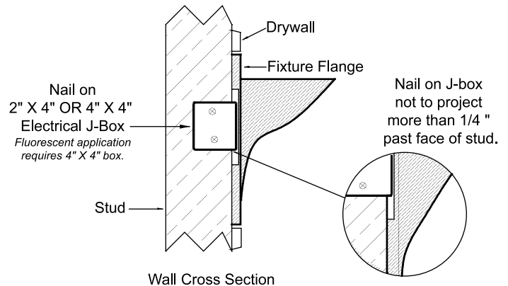
Wall Cross Section
